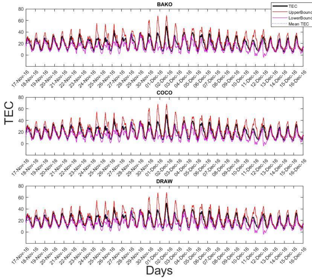
Fig. 2. 2 TEC from GPS stations (a) Bako (b) Coco (c) Draw related to EQ of M_w 6.5 Sumatra, for month of November and December (2016). The bold black line represents TEC. Red and Pink line represent the confidence bounds, while black dotted line indicates Mean Tec values before and after an EQ.
