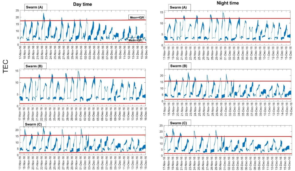
Fig. 3. 1 ionospheric anomalies from Swarm three satellites related to Sumatra EQ
